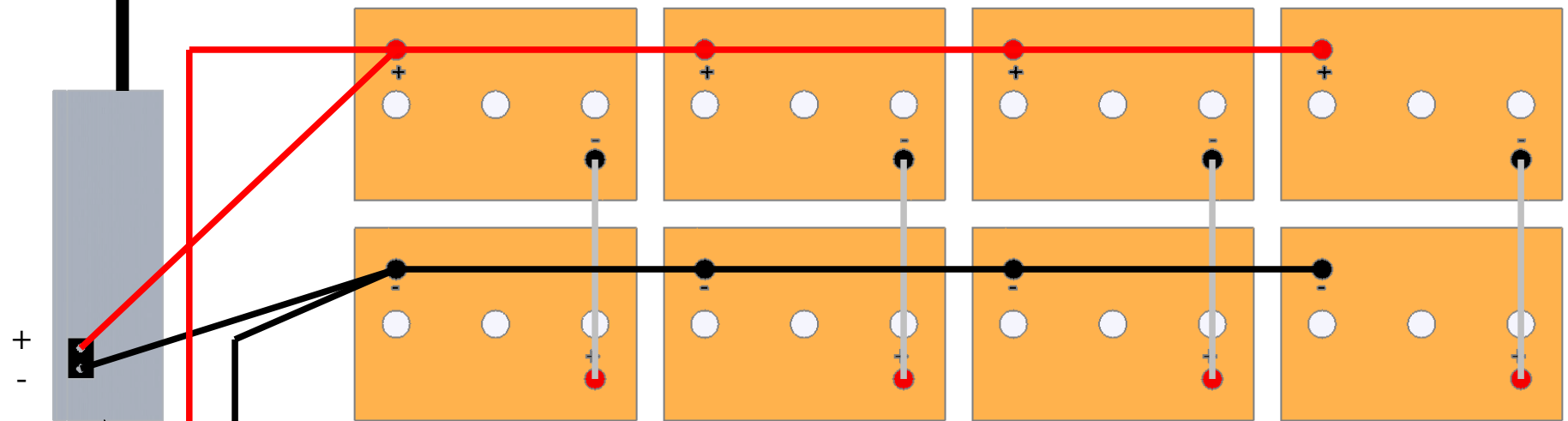
Battery Bank Of 6VDC Deep Cycle Batteries
